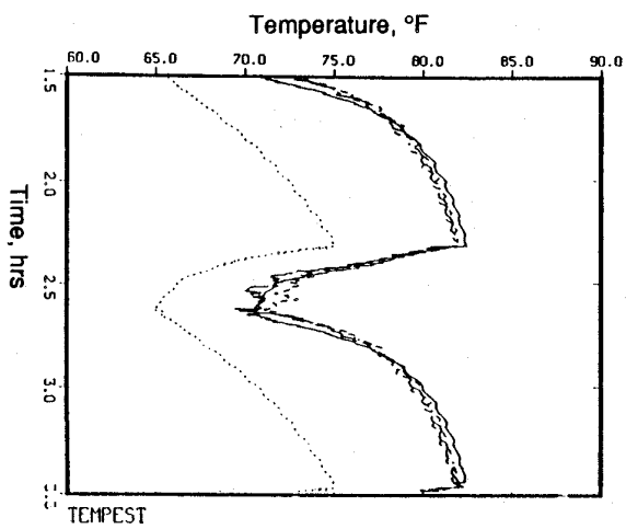
FIGURE 6. Case 4w Results
