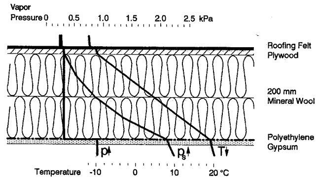
Fig. 4 The Glaser method applied to a flat roof construction exposed to an outdoor temperature of -12^{\circ}\text{C} . 6.1 \text{ g}/(\text{m}^2\text{-month}) condenses in the plywood.
