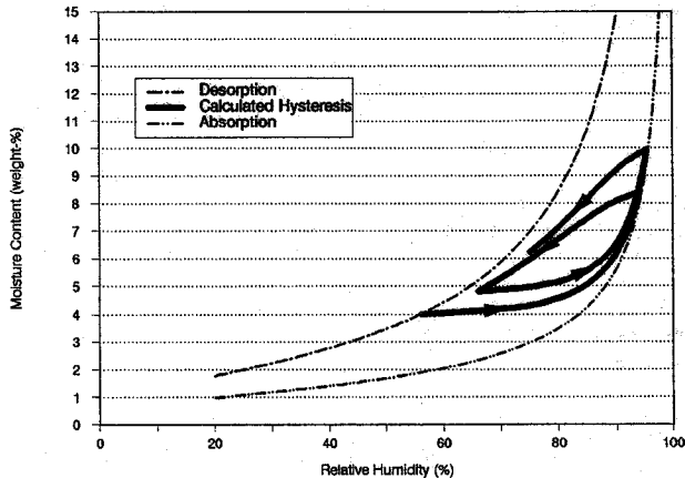
Fig. 1 Scanning curves followed in the sorption diagram for cellular concrete during interchanging periods of drying and wetting.
