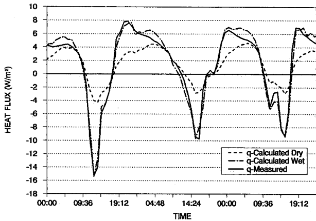
Fig. 3 Measured wet and calculated wet and dry heat flows for a fiber glass insulated roof construction with 0.25 vol-% moisture. Upward heat flow is positive.
