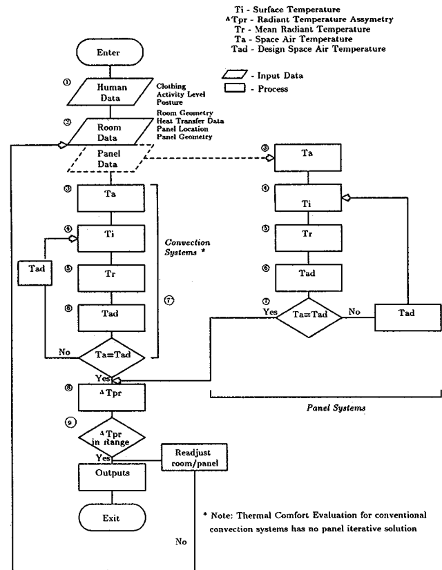
Figure 1 - Logic Diagram of the Thermal Comfort Design Method
