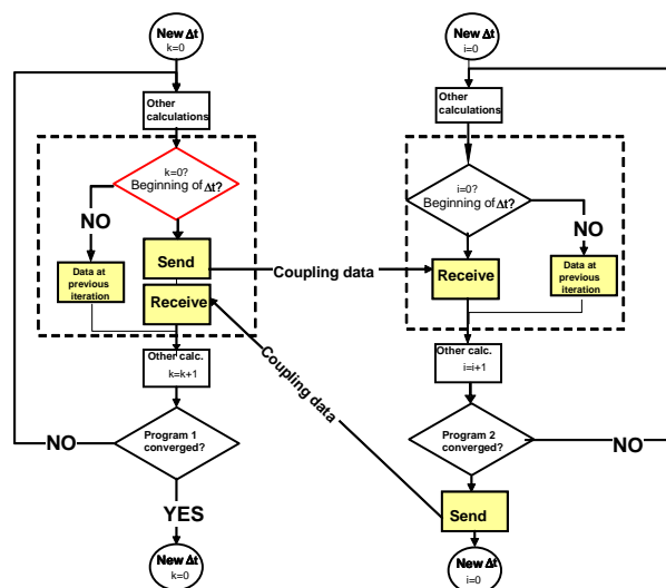
Figure 2: Flow-chart of loosely-coupled implementation. In our prototype, EnergyPlus takes the role of the program whose information flow is represented on the left side of the figure. The information flow of the second program corresponds to the TRNSYS role.
