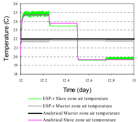
Figure 5 Zone air temperatures predicted by ESP-r program and analytical solution for the VAV control test.
