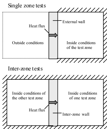
Figure 1 Comparison of test zones and boundary conditions in the single zone and inter-zone tests
