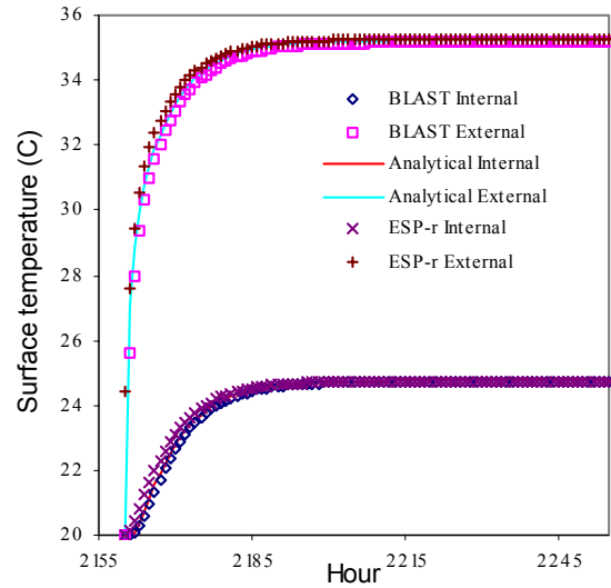
Figure 2 Analytically calculated surface temperatures and those predicted by BLAST and ESP-r for the inter-zone transient conduction test case with a conducting wall: first step change
