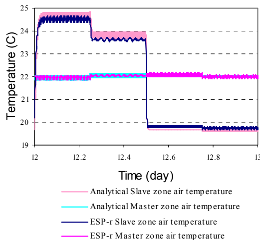
Figure 6 Zone air temperatures predicted by ESP-r program and analytical solution for the On-Off control test.
