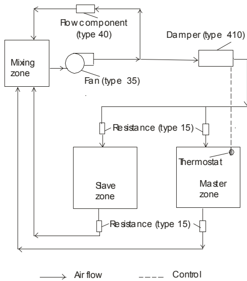
Figure 3 Airflow Network Used in ESP-r for VAV control tests with ESP-r program.
