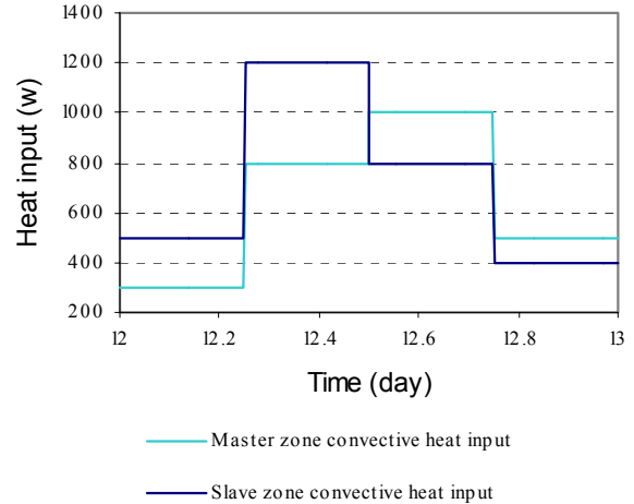
Figure 4 The convective heat input profiles of the test zones used in the VAV and On-Off control tests with ESP-r program.
