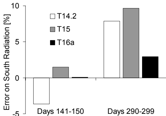
Figure 7: Error on radiation, South wall (IEA EV)
