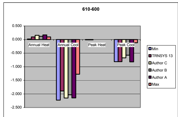
Figure 8: Sensitivity to South Overhang Shading
