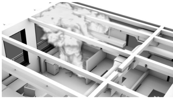
Figure 8: A volumetric rendering of hot buoyant plume.
