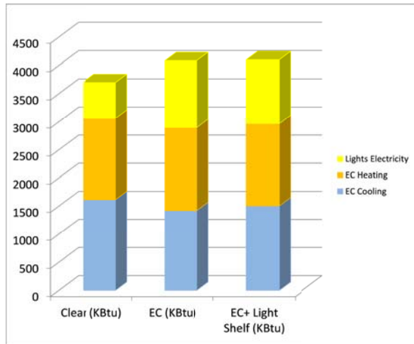
Figure 24: Cooling, Heating, Lighting Loads
